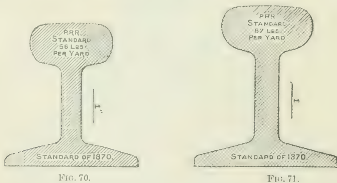
PENNSYLVANIA RAILROAD STANDARD RAILS, 1870.
