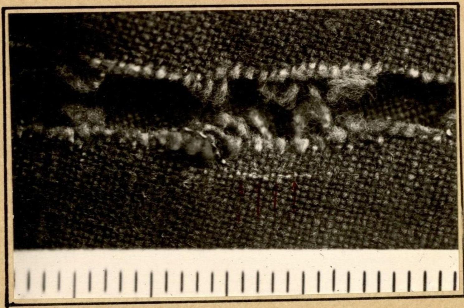
Photo N.10 Partial incision of filaments near the edge of the damages type 2
