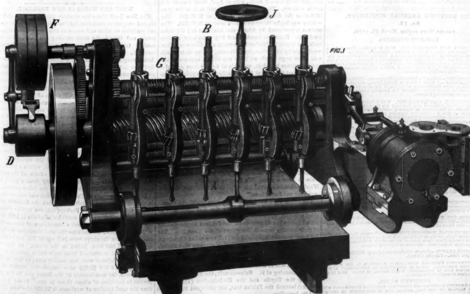
MULTIPLE DRILLING MACHINE.
