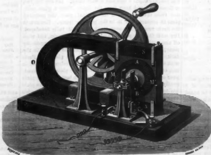
Fig. 5.—GRAMME'S MAGNETO-ELECTRIC MACHINE.
