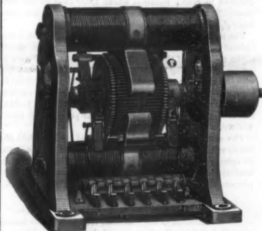
Fig. 6.—IMPROVED FORM OF GRAMME'S MACHINE.
