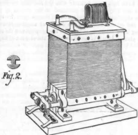
Fig. 2.—WILDE'S MACHINE, WITH SIEMENS' ARMATURE. are made with the Holmes improvement of the same machine.
