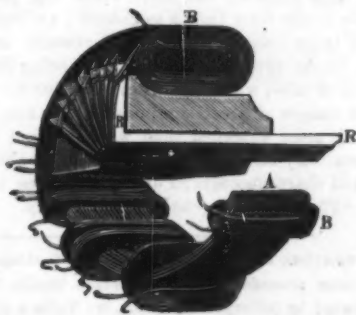
Fig. 4.—COIL OF GRAMME'S MACHINE.
