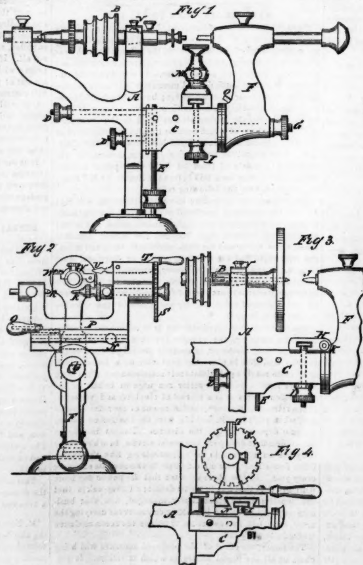
WILLIAMS' WATCHMAKER'S LATHE.
