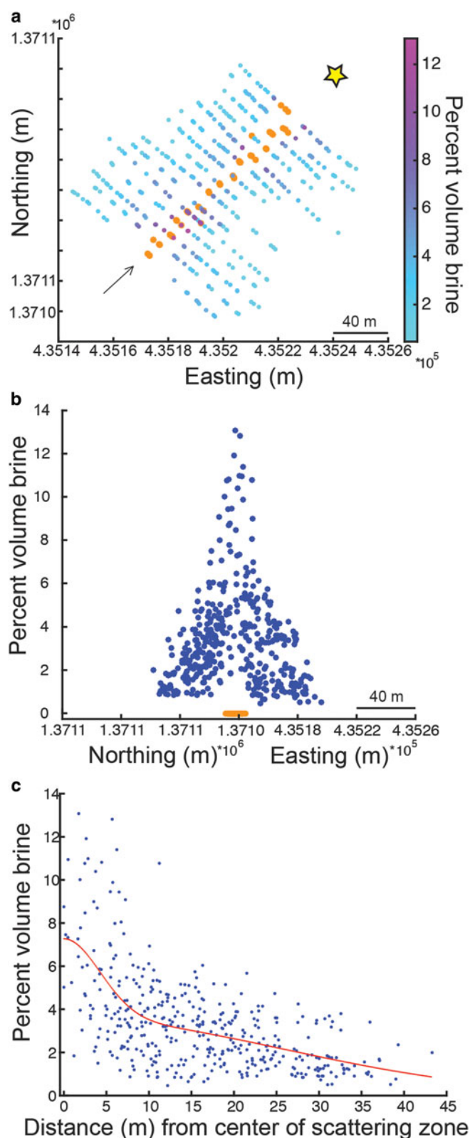
Fig. 6. Spatial variation of percent volume of brine using seawater as a proxy. (a) Map view showing brine content from low (light blue) to high (dark purple) in relation to the centers of the scattering zone for each transect (orange points). The star shows approximate location of the top of Blood Falls. The arrow gives reference for the orientation of part (b) along the central axis. (b) Along-arrow view from part (a) shows brine content on the vertical axis and the map plane on the horizontal axes. Orange points are the centers of the scattering zone for each transect. (c) Brine content as a function of distance from the center of the scattering zone (orange points) in each transect (note this distance reference is different than in (b)). The red line shows the two-part Gaussian model.
