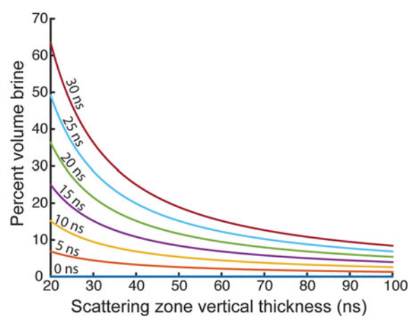
Fig. 7. The effect of scattering zone vertical thickness on the estimated brine content. Each line shows this effect for a different amount of downwarping in the underlying basal reflector (measured in one-way travel time).
