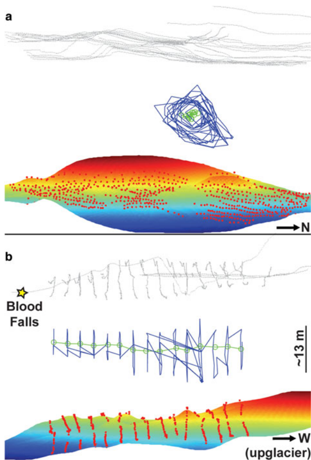
Fig. 5. Outline of scattering zone. The small black points identify GPS points used to define the glacier surface. Red points identify RES-picked points used to define the basal topography. Shading shows interpolated basal topography, with color denoting interpolated elevations (red is high and blue is low). Blue lines outline the scattering zone in each migrated RES transect. The green line connects the approximate centers of the migrated scattering zones on each transect defining the central axis of the scattering zone. (a) Subparallel to ice flow, this view of the scattering zone from Blood Falls looks up-glacier into the ice. (b) This cross-flow view of the scattering zone has Blood Falls to the left and looks across the glacier from north to south. Note that although these figures suggest a cylindrical conduit shape, this is solely a product of how we chose to define the edges of the scattering zone.
