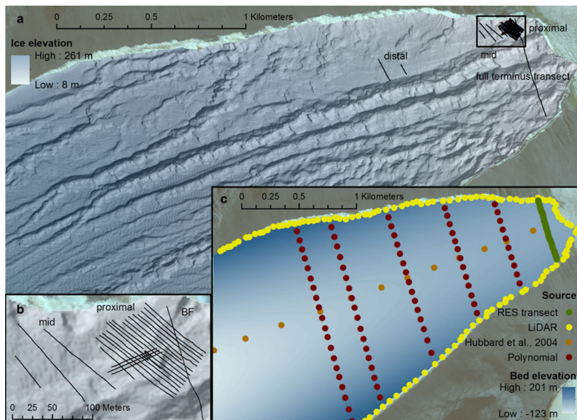
Fig. 2. Surface and bed topography of Taylor Glacier. (a) 2 m LiDAR digital elevation map from NASA/USGS (Schenk and others, 2004) with black lines showing RES transects. (b) Inset is an enlargement of the RES transect locations. BF marks the location of Blood Falls. (c) Calculated bed topography based on measurements (green circles are RES derived, yellow circles are LiDAR derived), approximations (orange circles are from analysis by Hubbard and others, 2004), and calculations (red circles are calculated hyperbolas derived from the LiDAR and Hubbard and others, 2004). Base map imagery from DigitalGlobe (2005).
