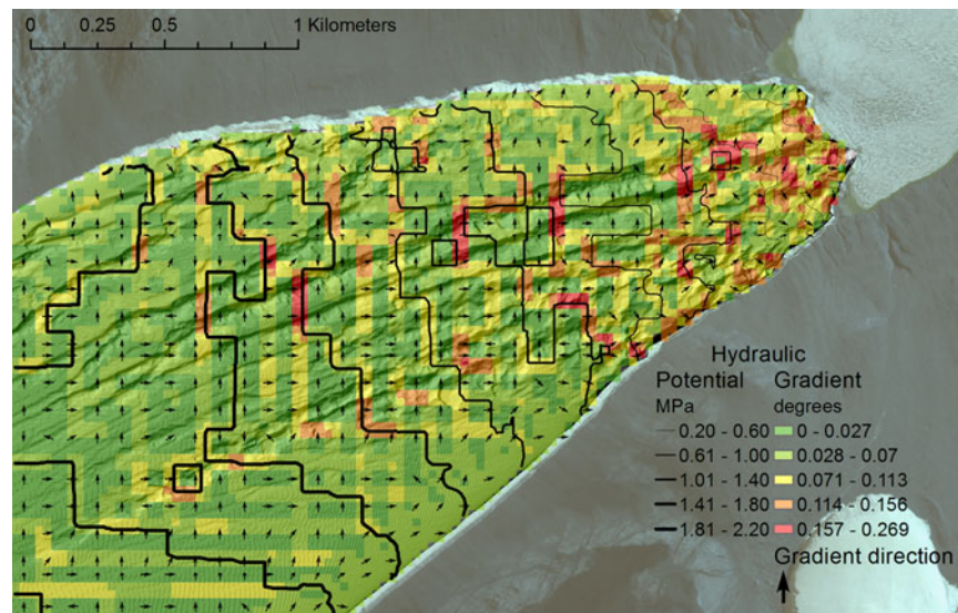
Fig. 8. Subglacial hydraulic-potential gradient model. This is an average of five trials in which each trial has artificial noise added to the bed topography (one standard deviation is 5%). The model varies resolution with estimated ice thickness. The hydraulic-potential gradient is calculated by the change in potential (MPa) over distance and is shown as high gradient (red) to low gradient (green). The arrows are a 90 m average gradient direction of the surrounding cells. The contours show hydraulic potential (MPa) from low (thin contours) to high (thick contours) potential. Base map imagery from DigitalGlobe (2005).
