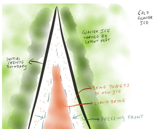
Fig. 10. Our proposed mechanism of basal crevassing explains the zone of englacial brine imaged by the RES. Spatially and temporally variable basal crevasses, most numerous near the center of the scattering zone, allow brine to inject into the glacier. Upon injection the brine begins to freeze causing latent heat of freezing to warm the surrounding ice and brine to become increasingly concentrated towards the center of the crevasse(s).
