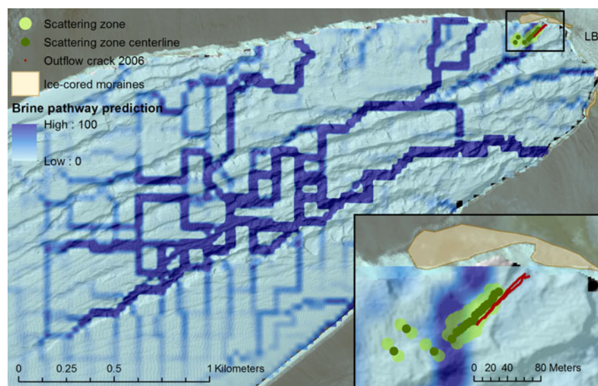
Fig. 9. Subglacial hydraulic-pathways predicted from hydraulic-potential calculation (Fig. 8). Darker blue indicates greater likelihood for brine flow channelization. The terminal ice-cored moraines (light brown), lateral extent (light green) and central axis (dark green) of the scattering zone, and 2006 brine outflow crack (red, personal communication T. Nylén) are shown and magnified in the inset. DigitalGlobe (2005) imagery shows the location of Lake Bonney (LB).
