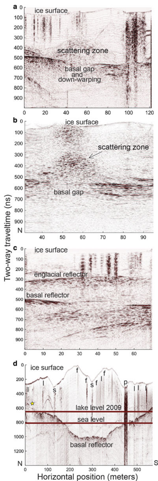
Fig. 4. Examples of topographically-corrected RES transects. (a) Unmigrated cross-flow transect from the proximal group showing the basal reflector, downwarping, and gap in the basal reflector and the scattering zone. (b) Cropped and migrated display of data in (a). (c) Unmigrated, along-flow transect from the proximal group showing the basal reflector as well as the englacial horizontal reflector referred to in the text. (d) Full-terminus transect showing the scattering zone (star) at the northern edge of the terminus. The basal reflector dips below the 2009 Lake Bonney water level and modern sea level (marked by red lines). The vertical reflections are marked by letters denoting the cause for the reflection: 'p' for meltwater pond, 's' for surface meltwater, 'f' for data file transition, 'l' for topographic low that collects meltwater.
