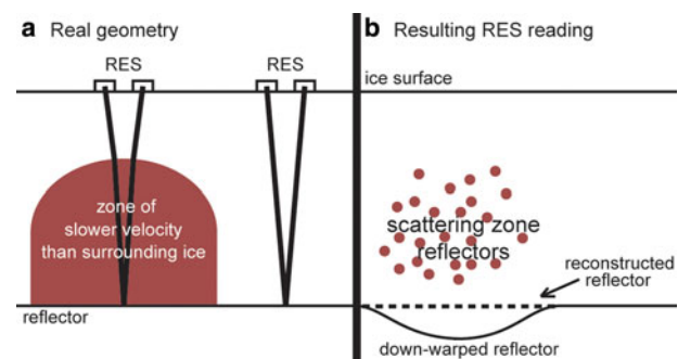
Fig. 3. Cartoon diagram of apparent reflector geometry as a function of differing ice properties. This illustrates a cause of the downwarping seen in Fig. 4a. (a) A geometrically horizontal reflector crosses under an englacial zone of water-rich ice. RES pathways pass through both the water-rich zone and the clean, meteoric surrounding ice. (b) The apparent geometry of the horizontal reflector, as imaged by RES, is affected by the slower velocity of electromagnetic waves through brine- or water-rich ice.
