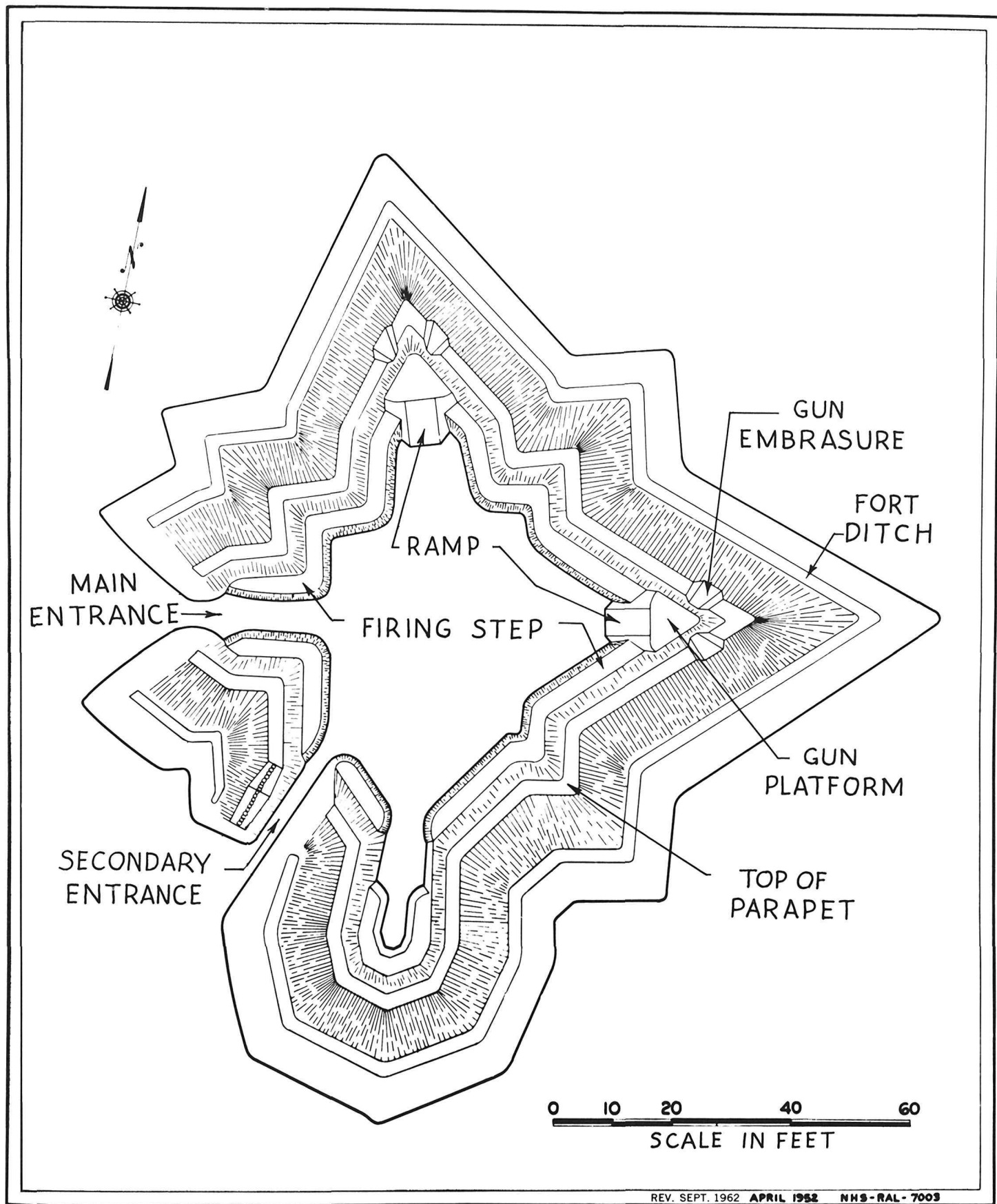
FIGURE 25—Plan of the fort as reconstructed
